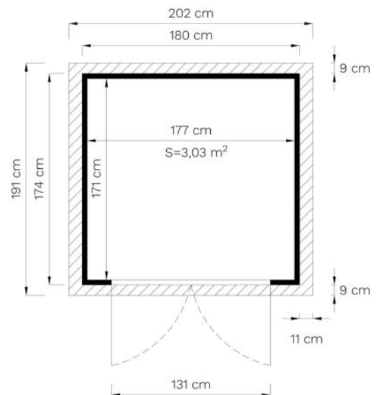
Fundamentplan / Foundation Plan
